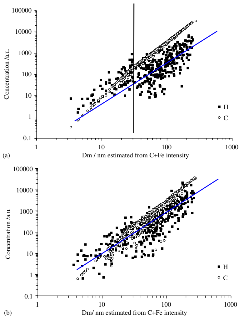
Fig. 10. Size dependence of carbon and hydrogen in diesel exhaust particles for the case of high-Fe doping: (a) 0 W load, and (b) 6 kW load. (Note: solid line through data shows D_{m,C}^2 dependence of elemental concentration.)
