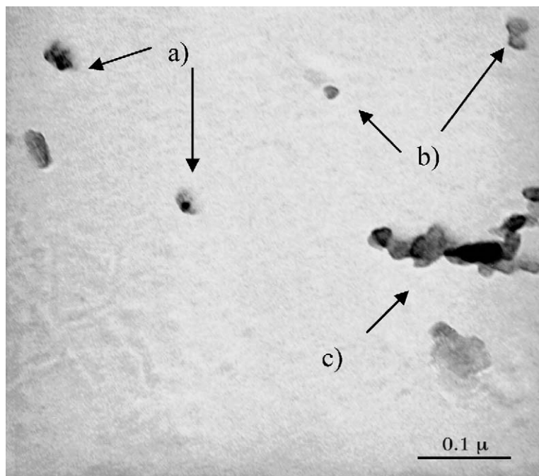
Fig. 7. TEM micrograph of size-selected DPM, showing: (a) nucleated iron particles, (b) hydrocarbon particles, and (c) chain agglomerate particle. Note: 6 kW load, 60 ppm iron doping rate.
