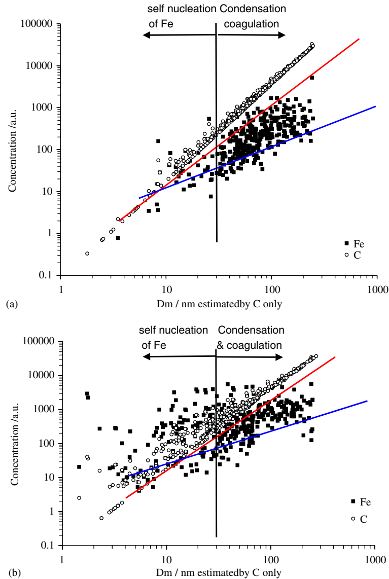
Fig. 11. Size dependence of iron and carbon fractions in diesel exhaust particles for the case of high-Fe doping: (a) 0 W load, and (b) 6 kW load. (Note that upper line shows D_{m,c}^2 while lower line shows D_{m,c}^1 .)
